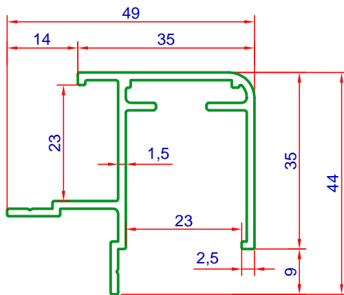
8603 0.620 kg/m
